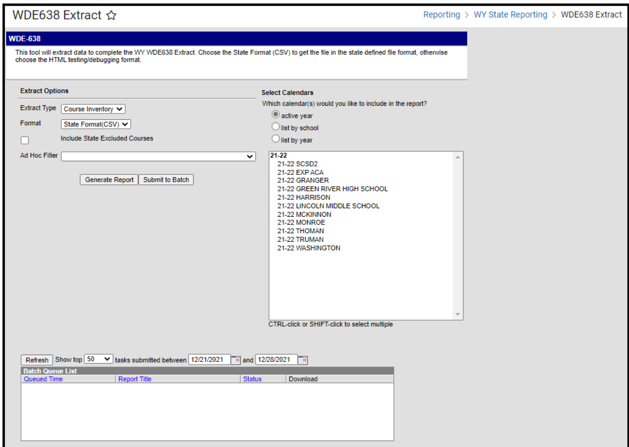
Image 1: Extract Editor
