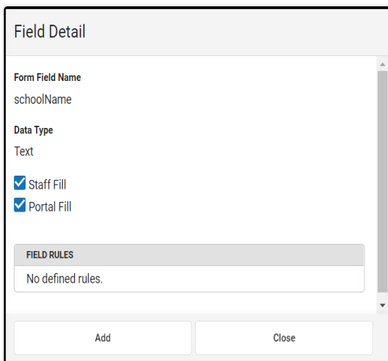
Image 21: Field Details
