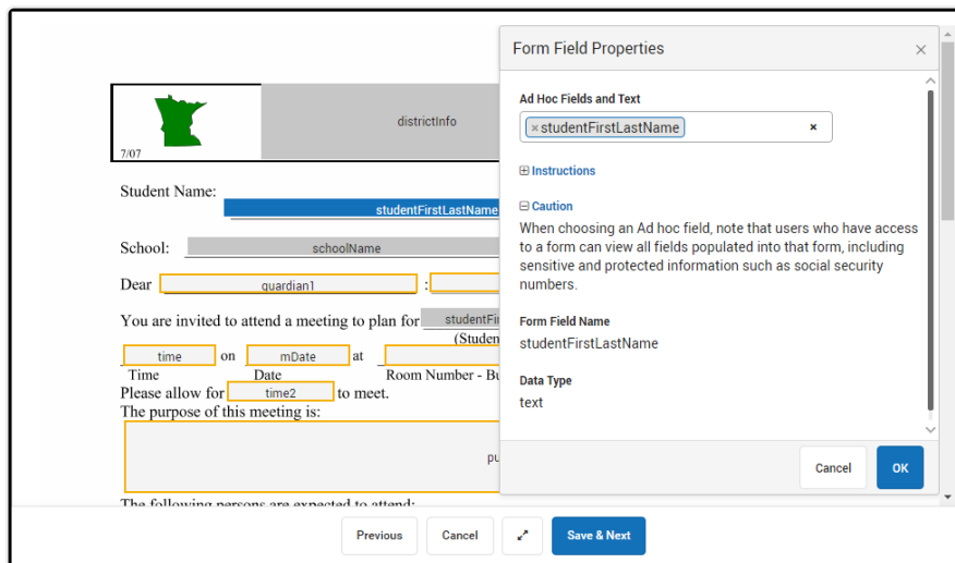
Image 9: Prepopulate Fields
