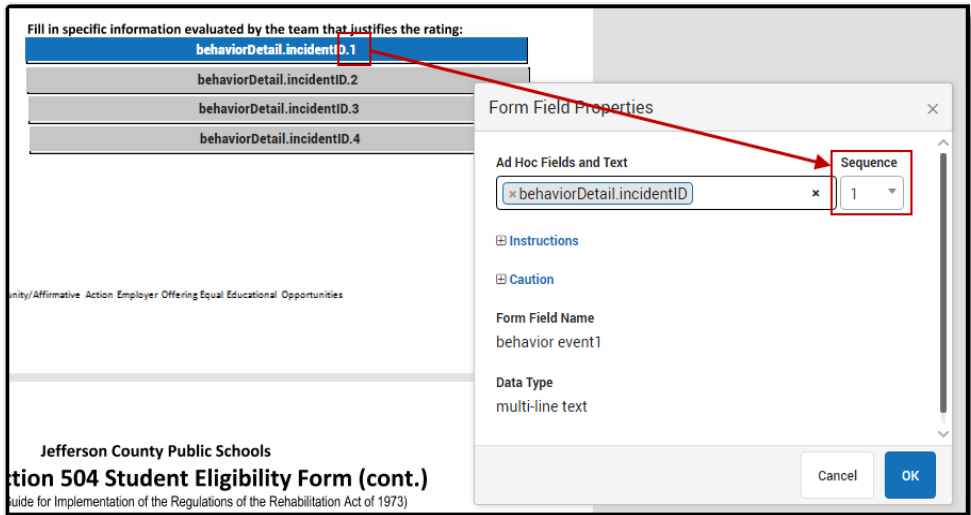
Image 10: Field Sequence
