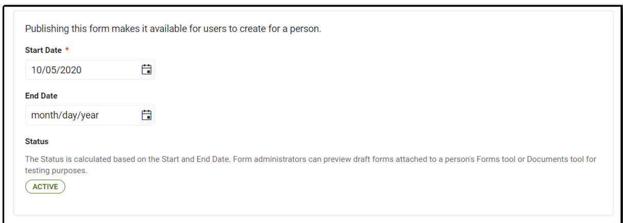
Image 29: Publish
