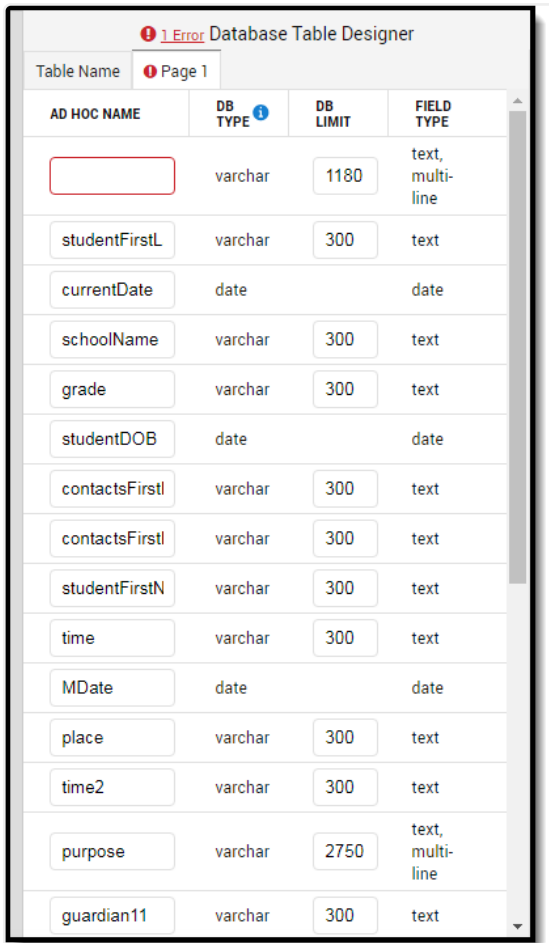
Image 14: Database Pagination
